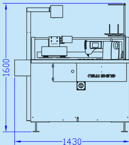
雙工位設計，可同時鋪料和車縫 Twin stations design for simultaneous operation of material placement and sewing
