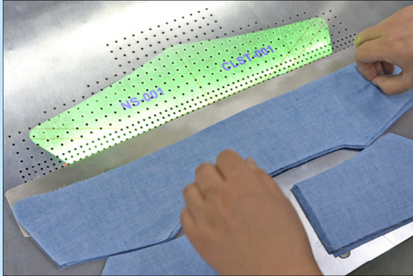
數碼投影裝置，鋪料對位更精準 Digital projector, enables accurate material placement
