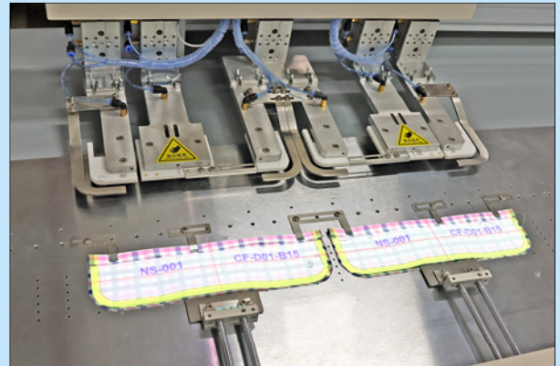
雙立體袖口同步操作 Double 3D Cuffs Synchronous Operation
